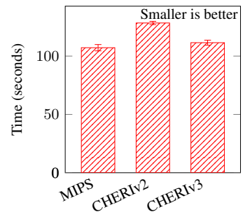
Figure 3. Tcpdump results
