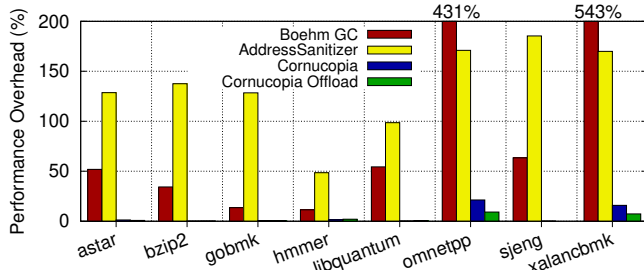
Fig. 5. Performance overheads for the Cornucopia snmalloc wrapper versus Boehm GC and AddressSanitizer executing on the MIPS FPGA platform. The baseline for Cornucopia is CheriABI, and the baseline for the others is MIPS. MIPS and CheriABI are generally within 5% of each other [13]. All benchmarks are run in their test configuration.
