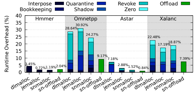
Fig. 4. Run-time overheads for revocation using a generic wrapper around dlmalloc , jemalloc , or snmalloc on the worst -performing, CHERI-compatible SPEC CPU2006 test workloads. The baseline is pure-capability execution without temporal safety. The fastest case is snmalloc offloading revocation to a separate thread. The offload case performs revocation without memory zeroing.
