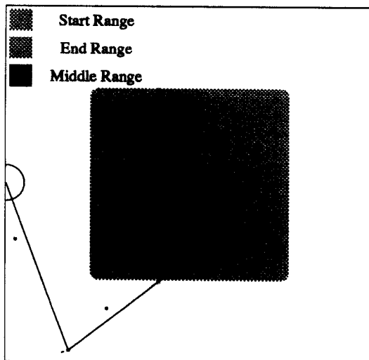
Figure 10.58: 5-d decomposed exploration. The arm starts randomly, from a 2-d set of states. The goal is chosen uniformly randomly from a 2-d set of states. The controller splits up the problem to reach the stationary middle state half way through path.
