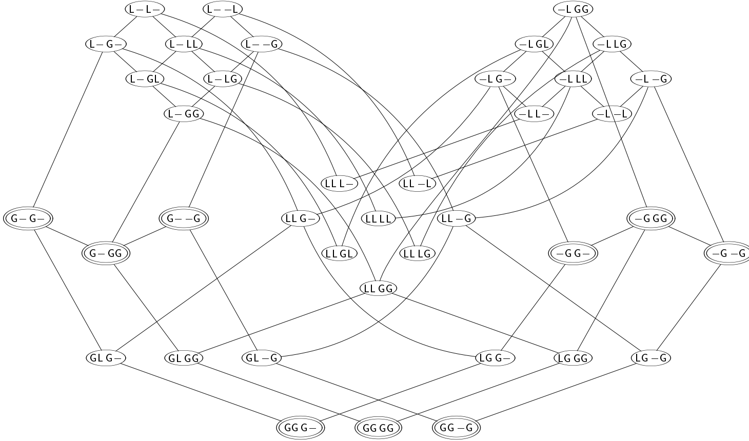
Figure 1: The subtype order over well-formed types \downarrow_{io} \downarrow_{i''o''} 1 . They are ordered by \downarrow_{io} \downarrow_{i''o''} 1 \leq \downarrow_{i'o'} \downarrow_{i'''o'''} 1 iff io \leq i'o' and o' = - \Rightarrow i'o' \leq i'''o''' , i' = - \Rightarrow i'''o''' \leq i'o' and o' \neq - \wedge i' \neq - \Rightarrow i'o' = i'''o''' .
